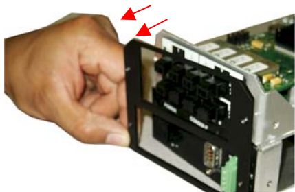
Figure 3.6.1d: Removing Face Plate
